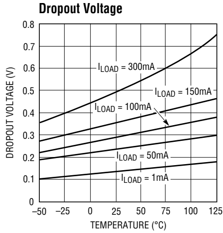
LT1521 • TPC02
