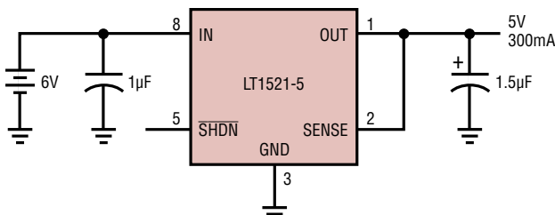
5V Battery-Powered Supply with Shutdown
